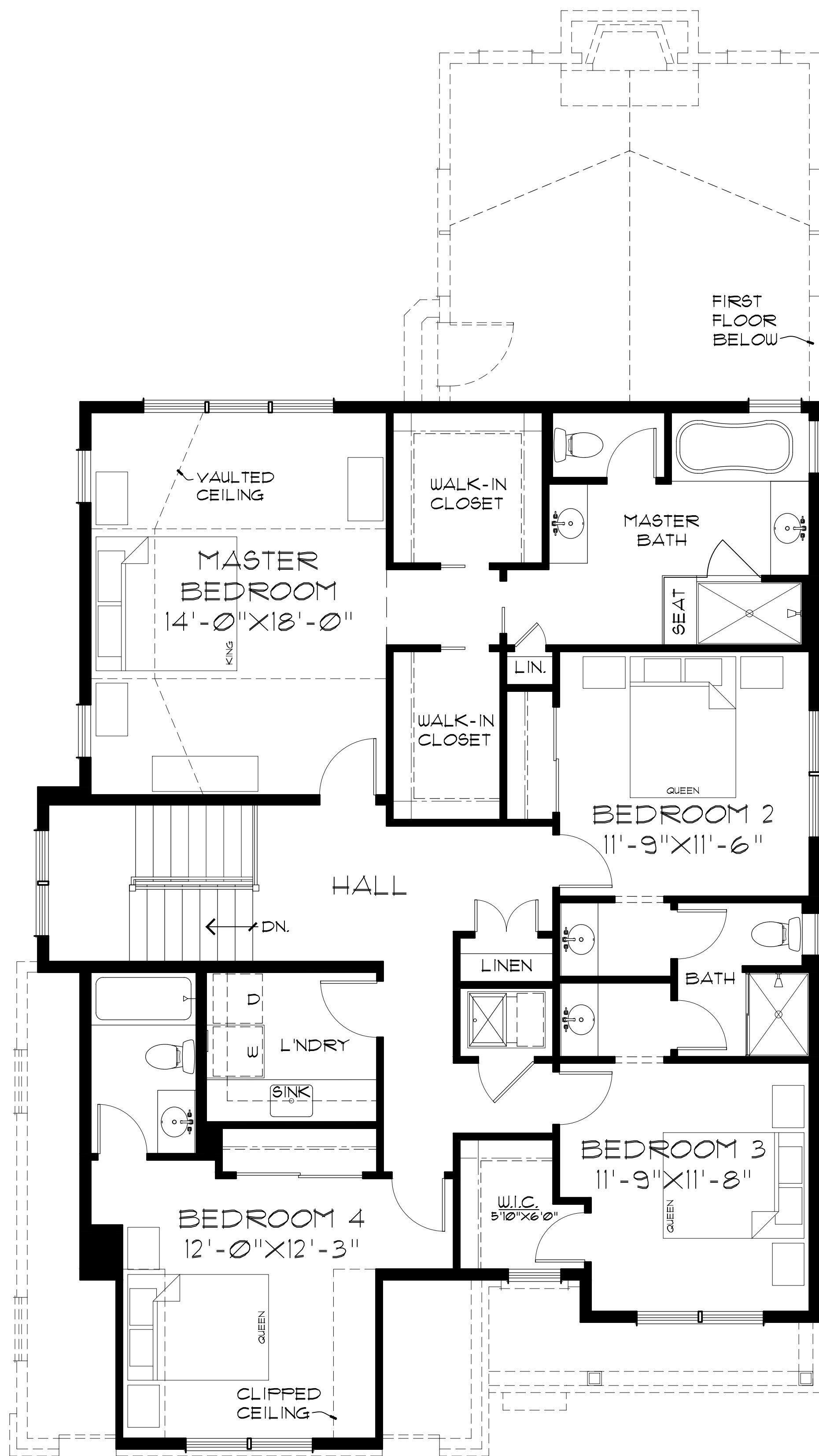
SECOND FLOOR 1,514 SQ. FT.
